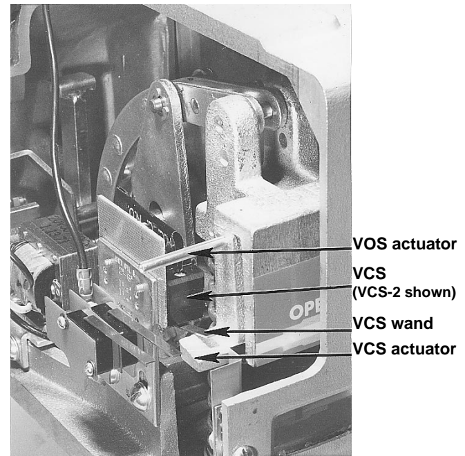
Valve Shut
