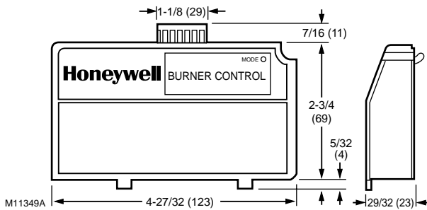
Fig. 1. Mounting dimensions of S7810M ModBus™ Module in in. (mm).
