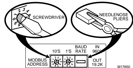
Fig. 4. S7810M Address Switches and Baud Rate Jumper.
